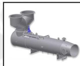
Exhaust gas heat exchanger, Pipings, bypass systems
